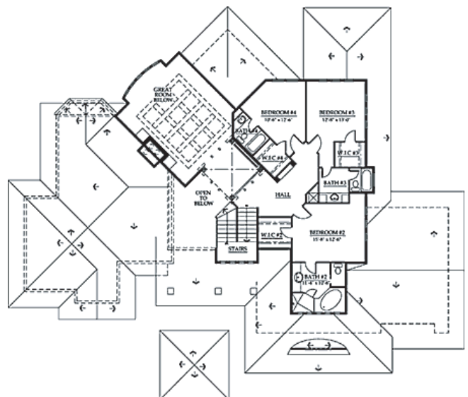
UPPER LEVEL 1278 SF
