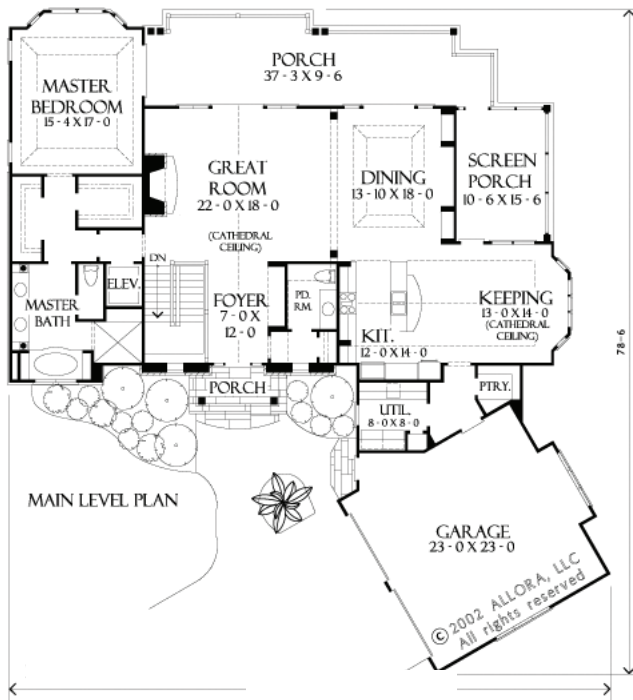
MAIN LEVEL 3201 SF
