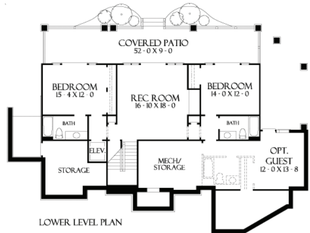
LOWER LEVEL 850 SF
