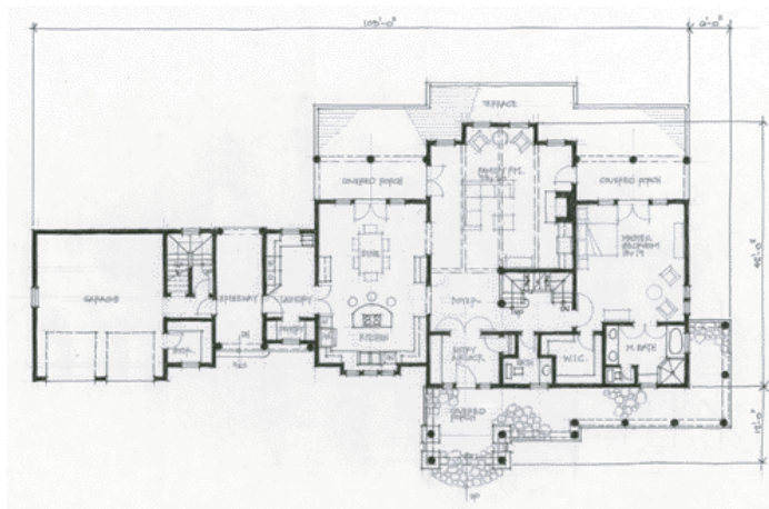
MAIN LEVEL 2160 SF
